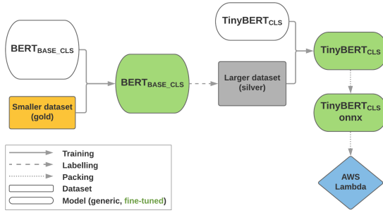
Figure 1: Schema of the distillation pipeline of BERT_{BASE\_CLS} for sentiment analysis. BERT_{BASE\_CLS} is fine-tuned on the gold dataset and then used for labelling a large amount of data (silver dataset) which serve as a training set for distillation to TinyBERT. The distilled model is exported to the ONNX format and deployed to AWS Lambda (see Section 5). The same pipeline was executed for MobileBERT.
